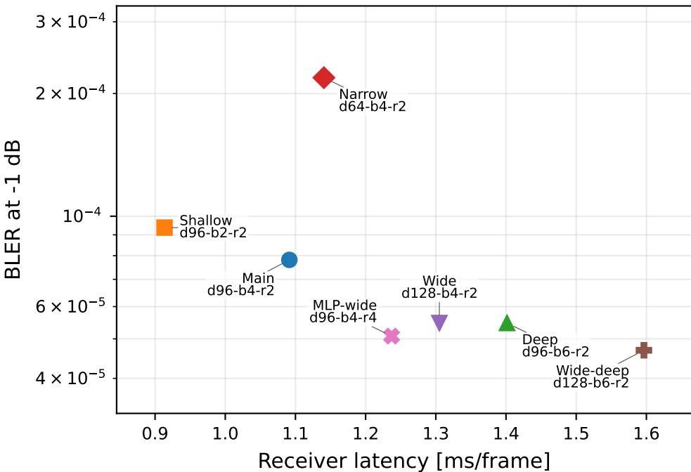
U2: accuracy-latency tradeoff
